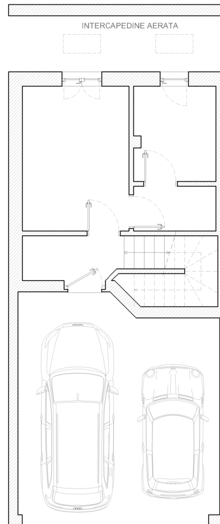
PIANO SEMINTERRATO*
