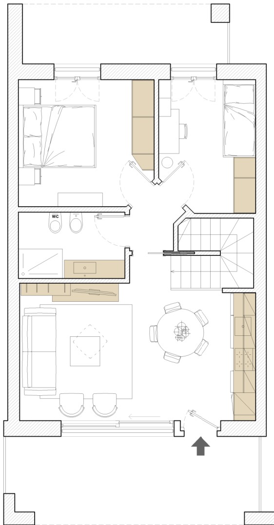
PIANO TERRA
